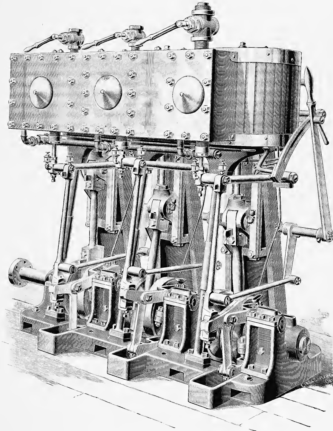
THE DAVIS-FARRAR TRIPLE-EXPANSION YACHT ENGINE, WITH DAVIS' RADIAL VALVE GEAR.
